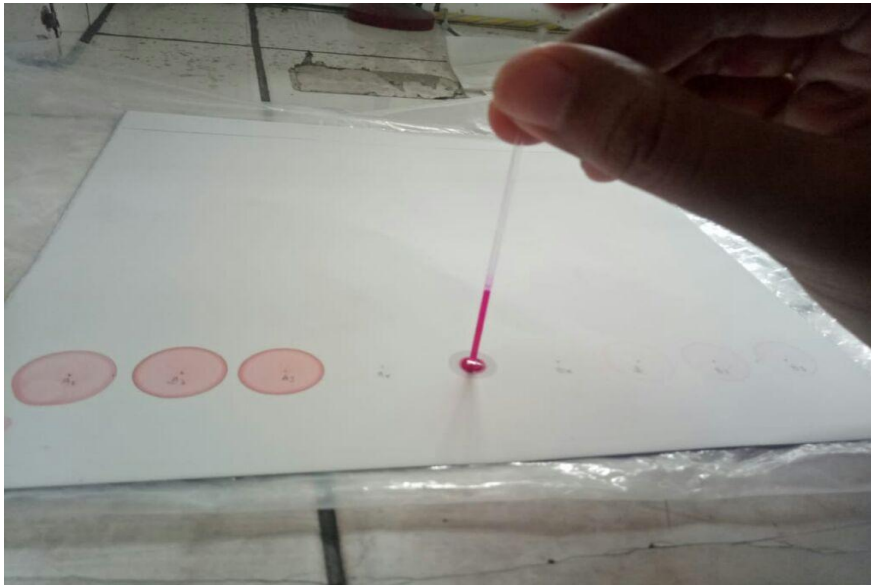
Gambar 6. Proses Penotolan
