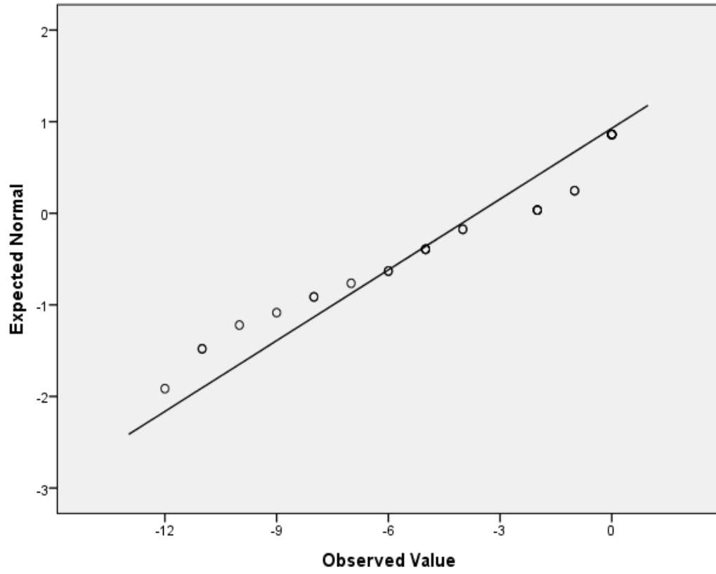
Normal Q-Q Plot of selisih
