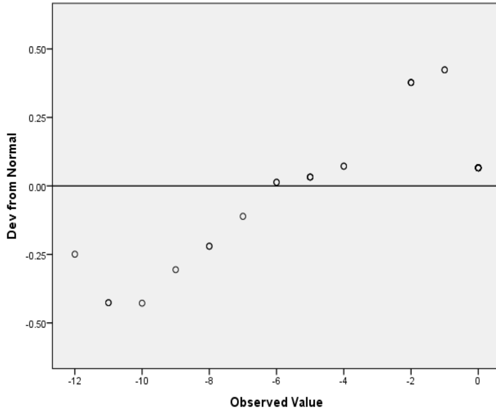
Detrended Normal Q-Q Plot of selisih
